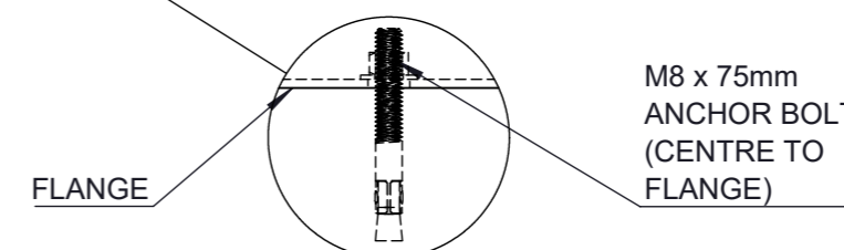
TYPICAL " BOLT DOWN" DETAIL
